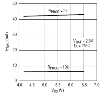
Trickle Charge Current vs Supply Voltage
