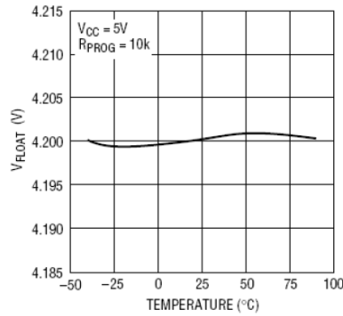
Regulated Output (Float) Voltage vs Temperature
