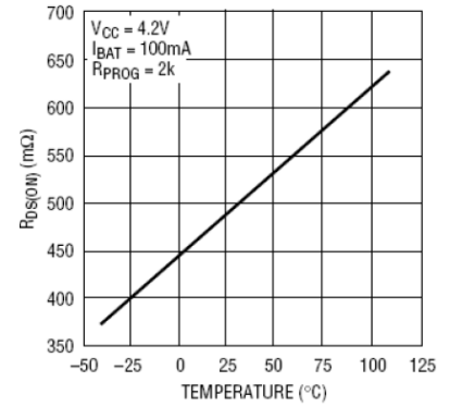
Power FET "ON" Resistance vs Temperature
