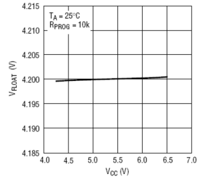
Regulated Output (Float) Voltage vs Supply Voltage
