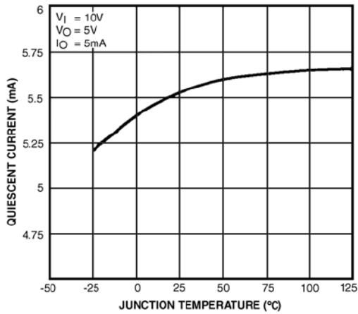
FIGURE 1. Quiescent Current
