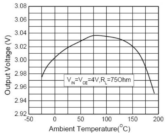
Figure 10. Output Voltage vs. Ambient Temperature
